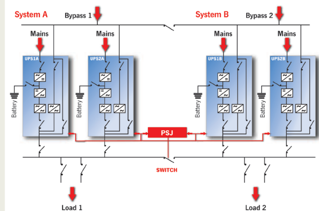
Konfiguration Dual Bus
